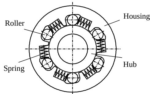
Figure 1. Roller freewheel assembl
