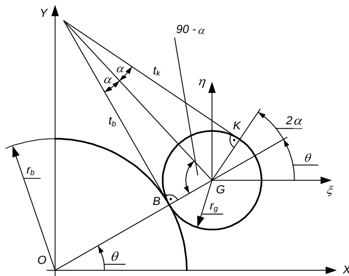
Figure 5. Layout draft of the roller freewheel
