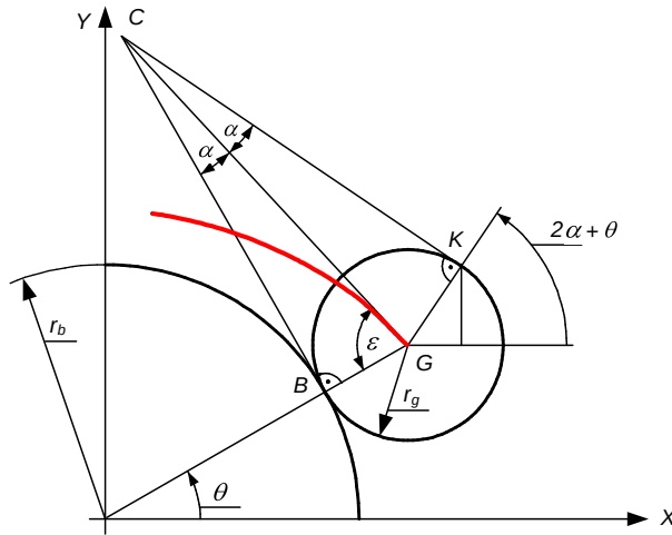
Figure 6. Moving of the roller central point
