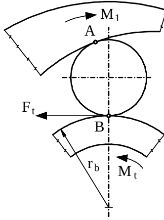
Figure 3. The operating principle of the roller freewheels
