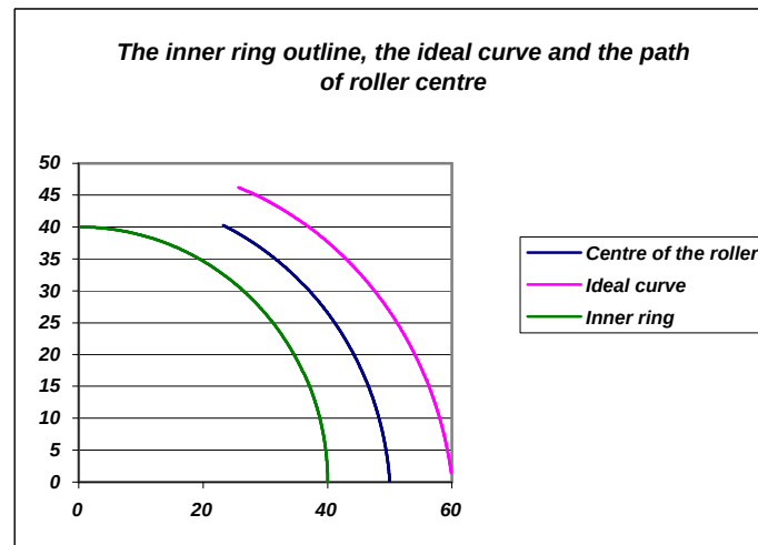
Figure 7. The inner ring outline, the ideal curve and the path of roller centre
