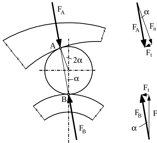
Figure 4. The equilibrium of forces acting to the roller
