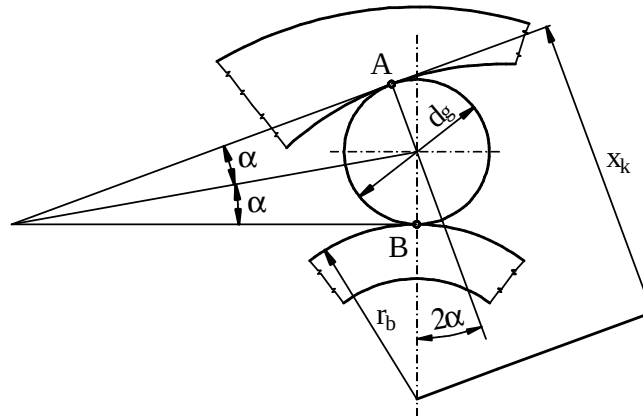
Figure 2. The geometry of the contact
