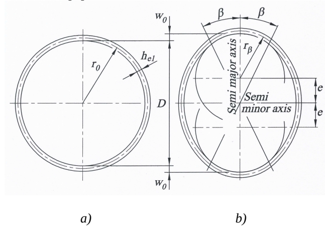
Figure 3. a) Ring substituting the flexspline b) Ring deflected by two disks with eccentric bearing support
