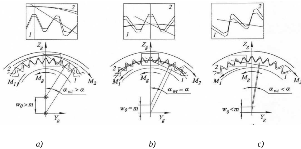
Figure 5. The location of meshing teeth in relation to the semi major axis of the wave generator as the function of radial deflection, w_0
