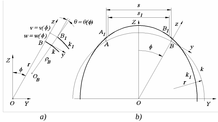
Figure 1. Arcuation. a) The displacement of an arbitrary point and b) the change in chord length
