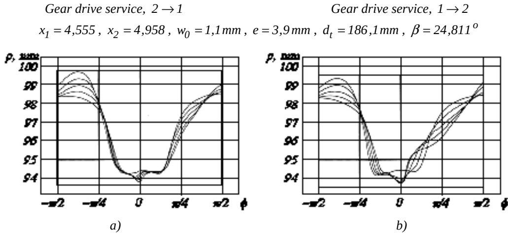
Figure 11. The radius of curvature, in the function of deviation relatively to the major axis
