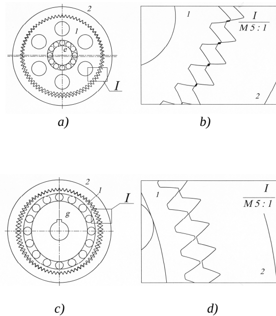
Figure 2. a) and b) Planetary gear drive, c) and d) Harmonic gear drive
