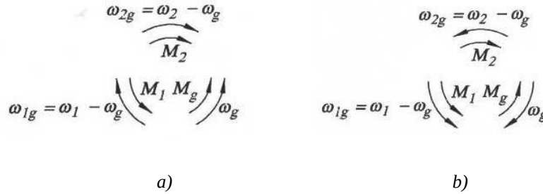
Figure 9. Torques acting to the elements of the drive and the angular velocities in gear drive service.
