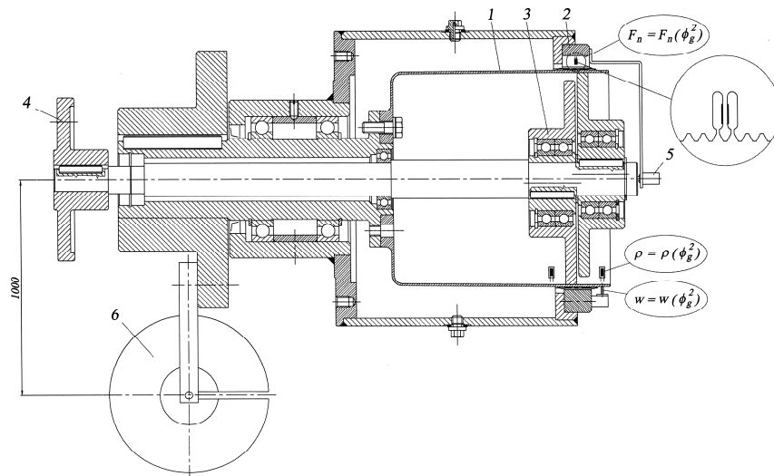
Figure 7. Experimental drive. 1 flexspline, 2 circular spline, 3 wave generator, 4 coupling, 5 rotating transducer, 6 loading disk
