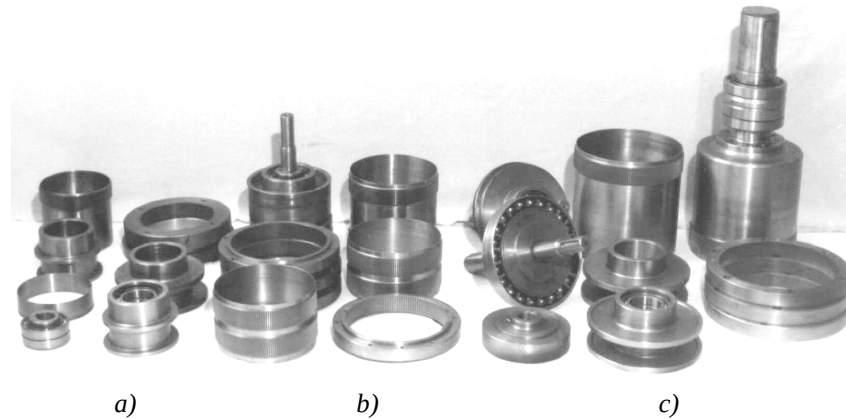
Figure 6. Basic elements of the Harmonic drive. a) ND120 , b) ND160 , c) ND190 drive elements
