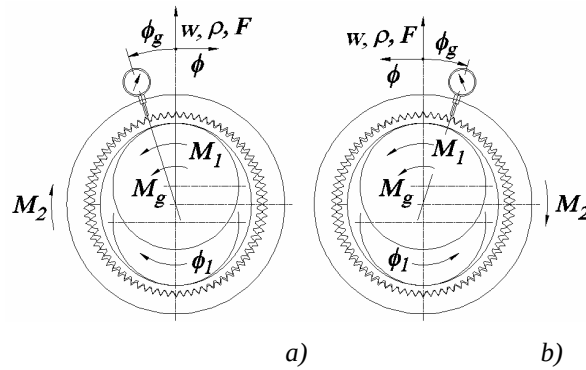
Figure 8. The wave generator deviation and the recording of measured amounts in harmonic gear drive service. a) The harmonic drive slows down, b) speeds up
