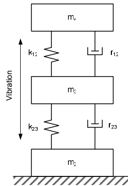
Figure 4. Mechanical model of rolling bearing
