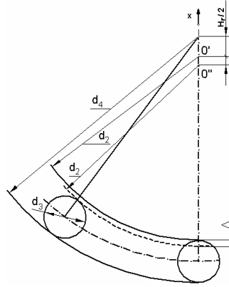
Figure 5. Seat evolved on one or two rolling body caused by the internal clearance of rolling bearings
