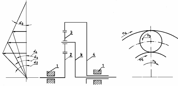
Figure 6. Rolling bearing substituted by planetary gear for defining revs
