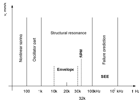
Figure 9. Suggested measuring methods in different frequency intervals [4]
