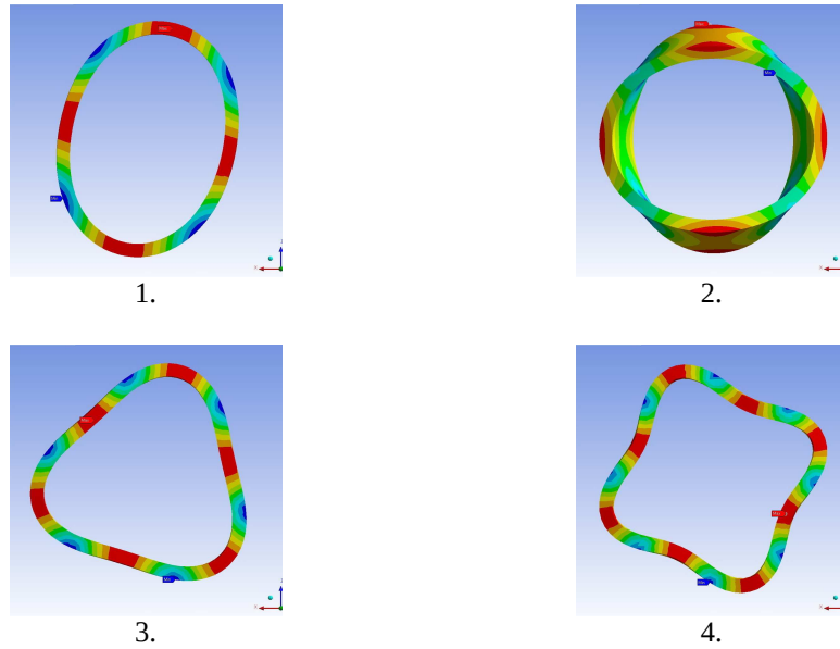
Figure 8. Resonance shapes of Eigen frequencies in case of rolling bearing rings (first 4)
