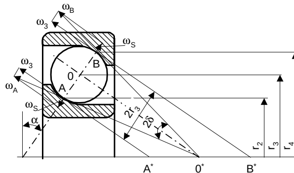
Figure 7. Sketch of an angular contact ball bearing
