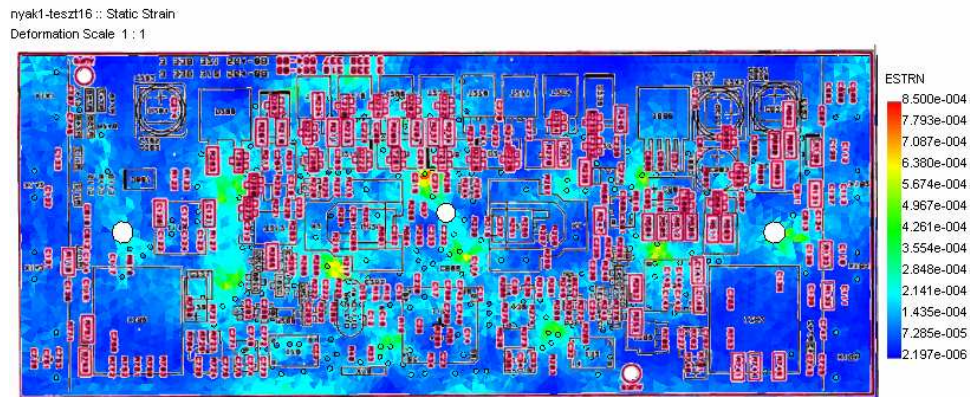
Figure 2. Strain contours shown on the assembly plan of electronic elements. This picture helps to decide which electronic element is in dangerous position
