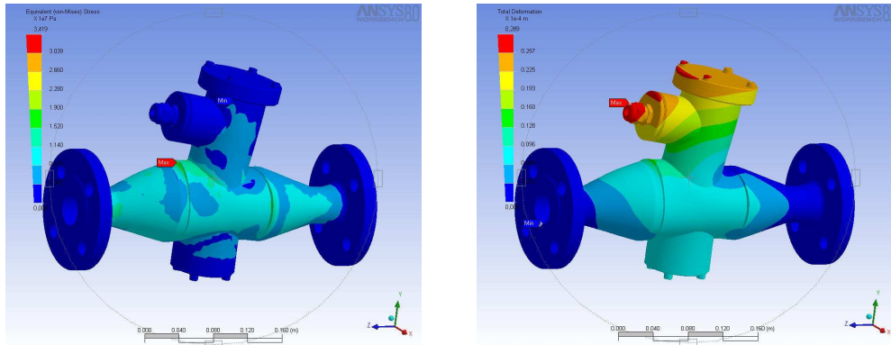
Figure 4. Stress (to the left) and deformation (to the right) contours of the igniter
