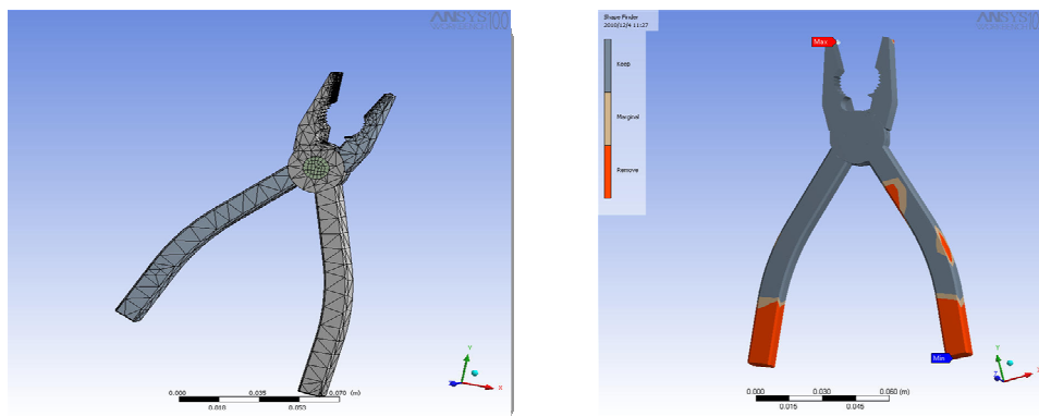
Figure 5. a) (Initial shape) and Figure 5. b) (materials to eliminate) of pliers model
