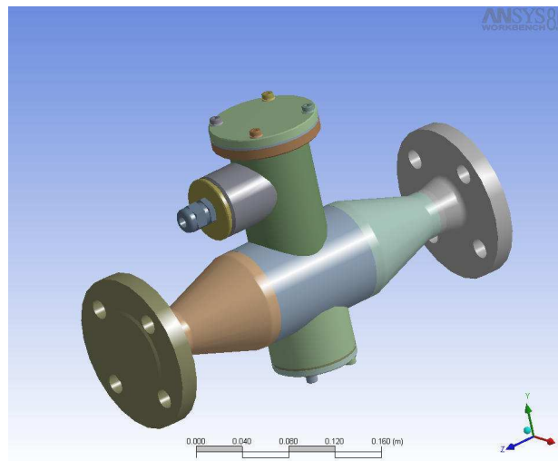
Figure 3. The igniter chamber
