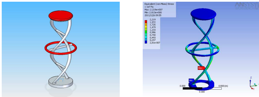
Figure 7. a) Original shape of the bar- chair and Figure 7. b) stress contours under the load caused by a sitting person
