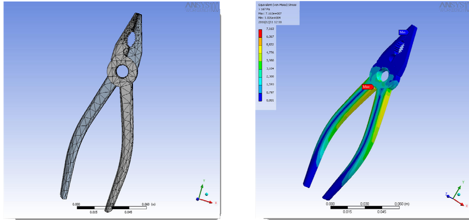
Figure 6. a) (New, improved form) and Figure 6. b) (Stress state verification) of the product
