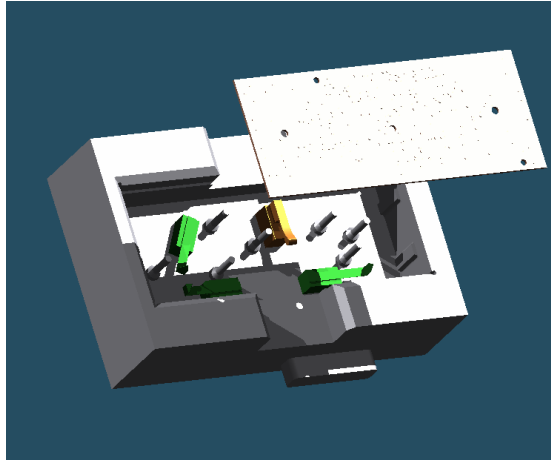
Figure 1. Supporting pins and the assembly of the panel into the measuring frame
