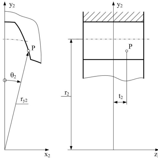
Figure 7. Tooth surface of internal gear
