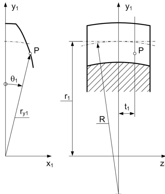
Figure 5. Crowned tooth surface
