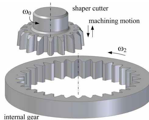
Figure 6. Gear shaping of an internal gear
