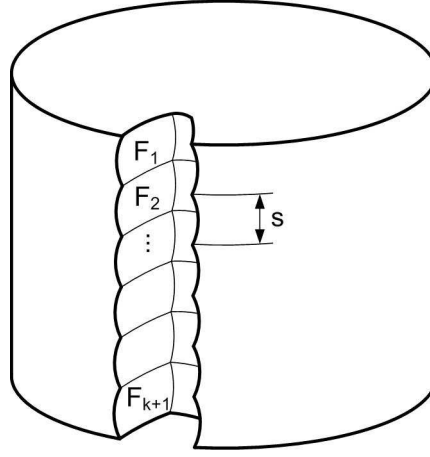
Figure 4. Real tooth surfaces of a cylindrical spur gear
