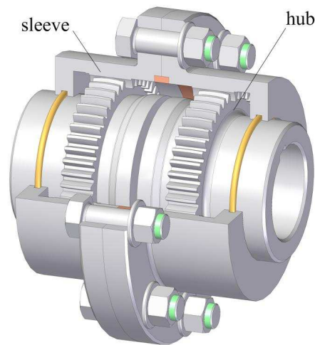
Figure 1. Gear coupling
