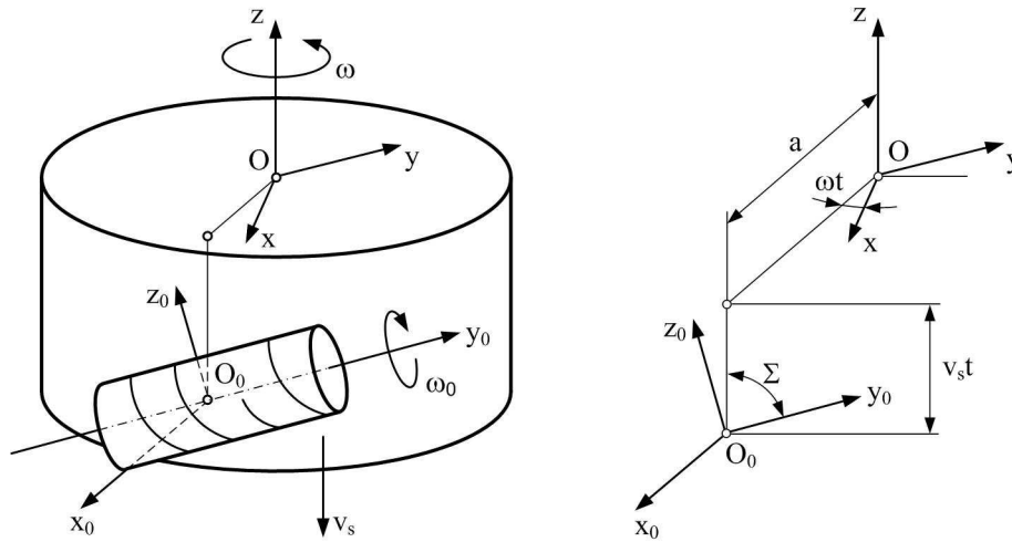
Figure 3. The sketch of hobbing and the used coordinate systems
