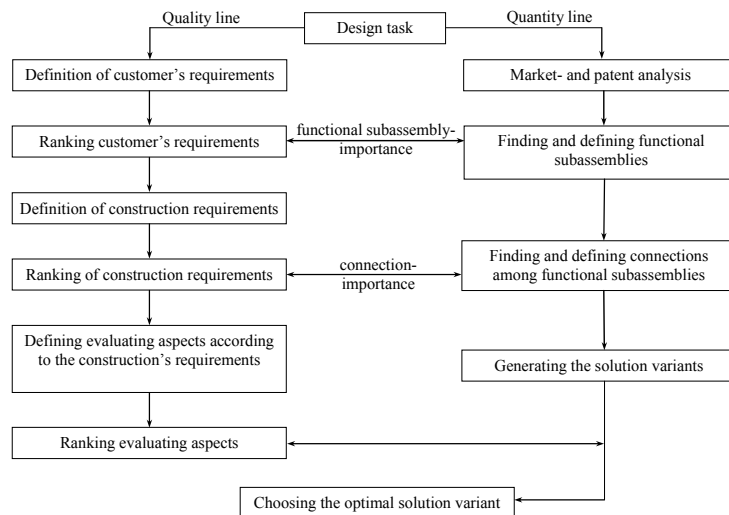
Figure 2. Logical steps of the suggested computer aided concept building
