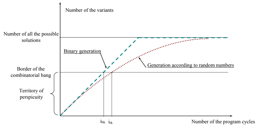
Figure 4. The maximum number of solution variants according to the binary logics and the theory of random numbers
