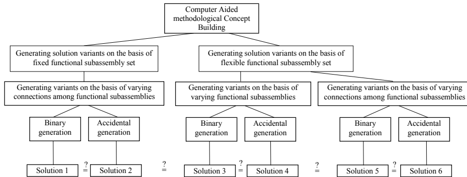
Figure 3. Generating solution variants
