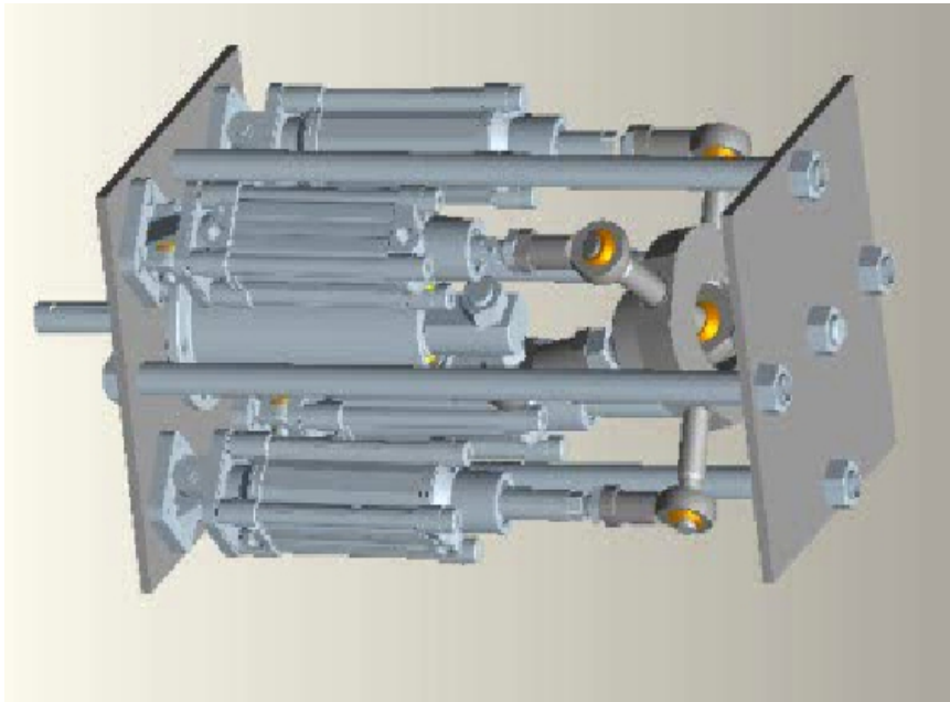
Figure 4. Tottering disk pneumatic motor (2 kW & 10 bar and 95 1/min)
