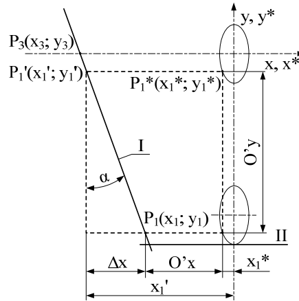
Figure 3. Tool basic profile with ellipse curve [4]
