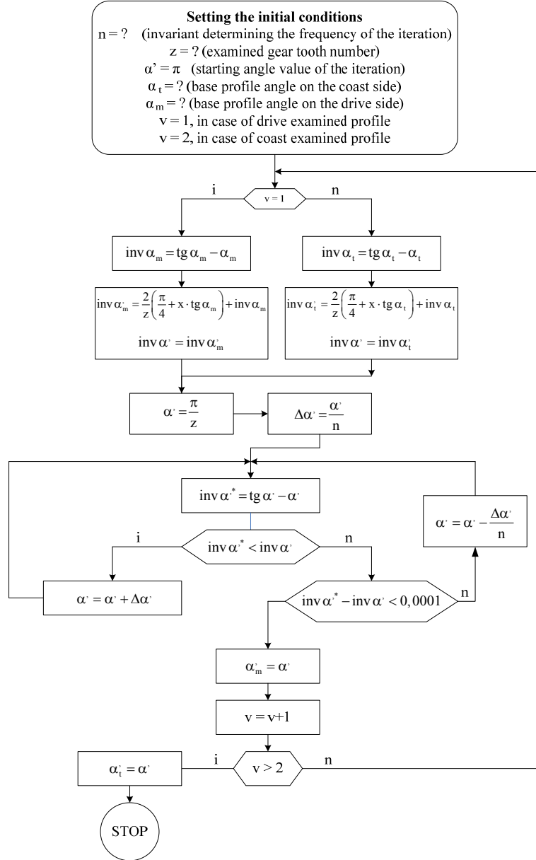
Figure 6. Angles belonging to the closing of the tooth profile sides
