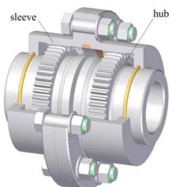
Figure 1. Gear coupling
