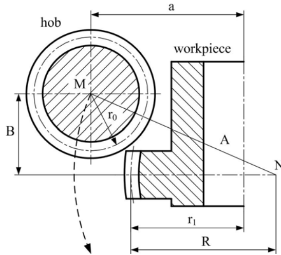
Figure 2. A conceptual sketch for manufacture of crowned tooth surfaces
