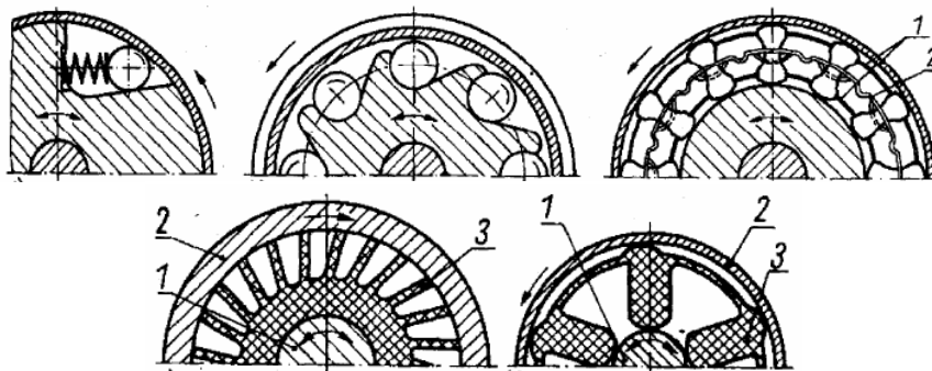
Figure 3. Free-running clutches – wedging rigid roller type, closure body type and elastomer disk type [4]
