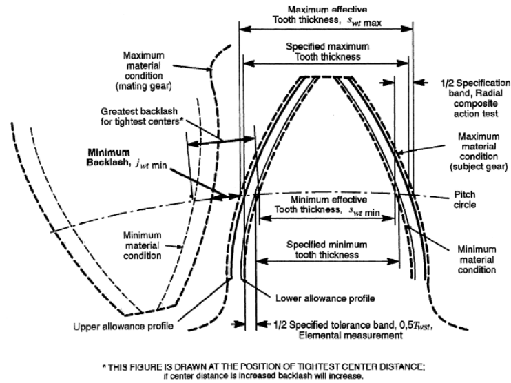
Figure 2. Tooth thickness, transverse plane [2]
