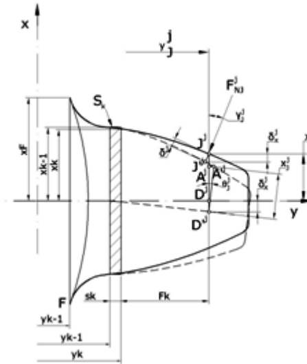
Figure 7. Model of the tooth
