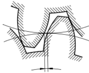
Figure 3. Circumferential backlash [1]
