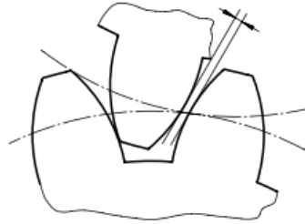
Figure 4. Normal backlash [1]
