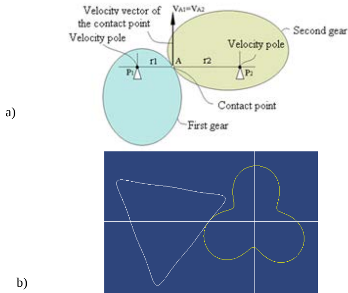
Figure 5. a) Sketch for the evaluation of the curves b) apairs of rolling curves
