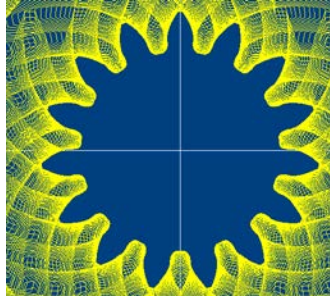
Figure 8. The standard profile rolled on a circle
