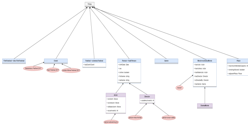
Figure 6. Visualization of FilmFestival in RelOntoUML
