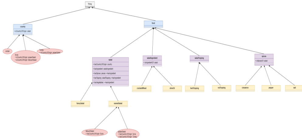
Figure 8. Visualization of Funny Salad in RelOntoUML
