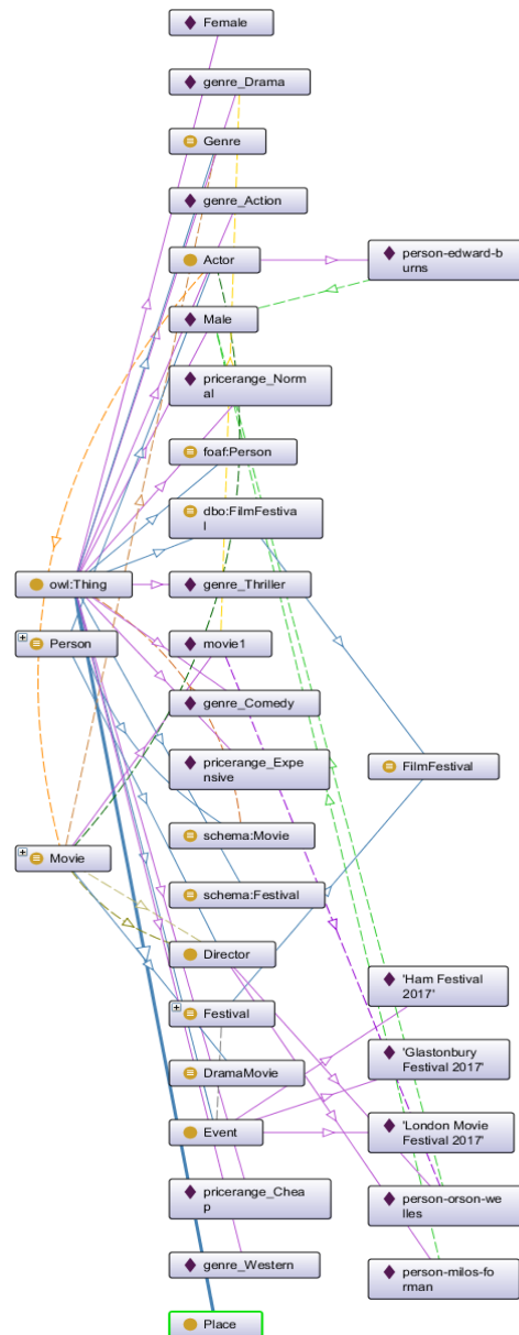
Figure 5. Visualization of FilmFestival in OntoGraf
