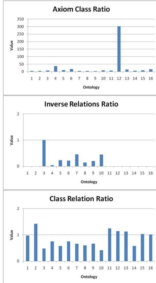
Figure 7. The schema axioms
