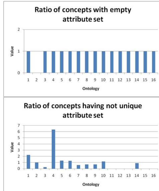
Figure 10. The attribute-oriented metrics
