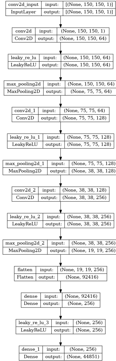
Figure 2. CNN model
