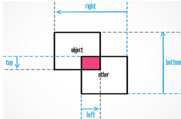
Figure 4. AABB collision
