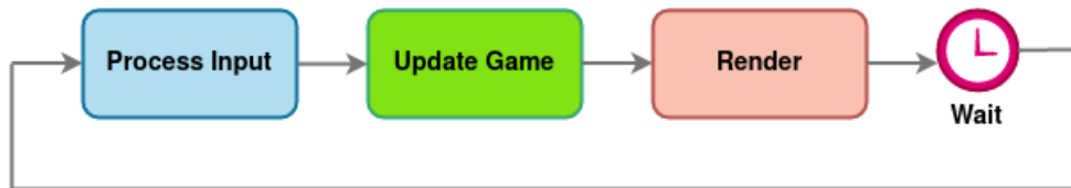
Figure 1. Fixed-time step loop
