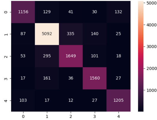
Figure 3. Confusion matrix for RNN-LSTM
