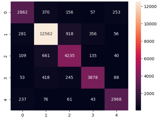
Figure 5. Confusion matrix of MLP
