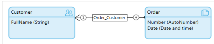
Figure12. Two entities with an n/1 association
