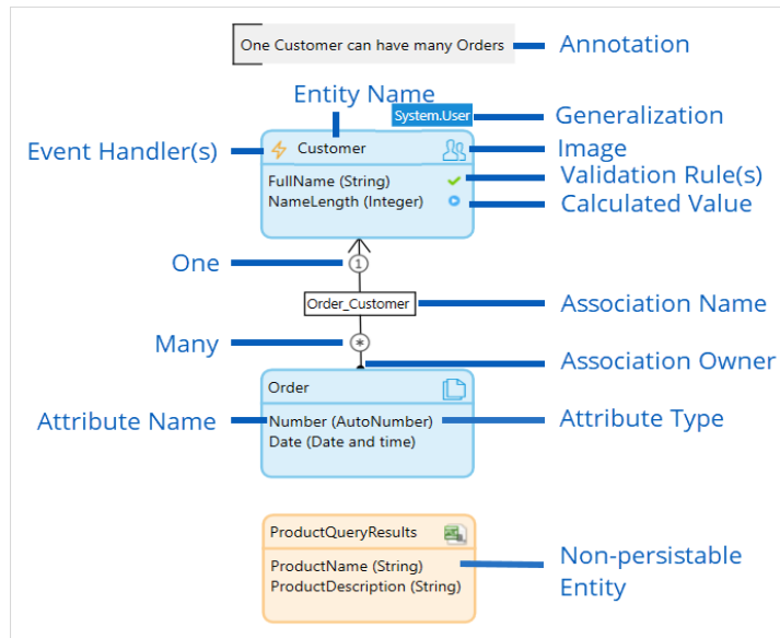
Figure 13. Domain model that defines customers and orders [Source: Mendix Docs]
