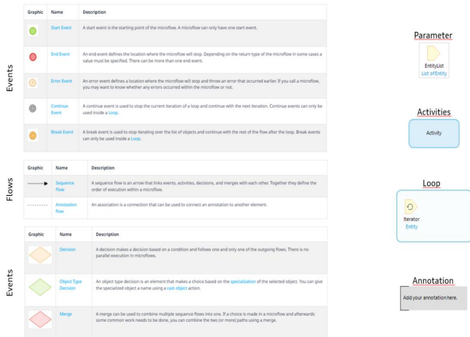
Figure 18. Standardized graphical notation of all components [Source: own]
