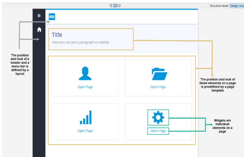
Figure 14. Page layout [Source: Mendix Docs]
