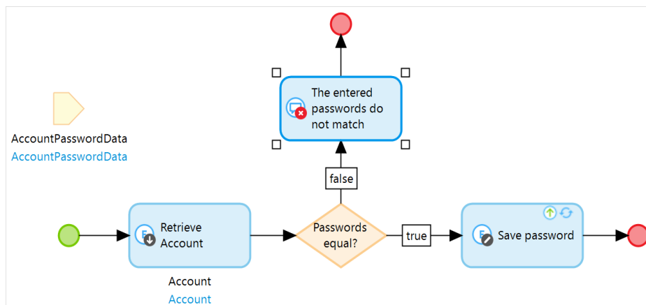
Figure 17. 'Retrieve Account' Microflow [Source: Mendix Docs]
