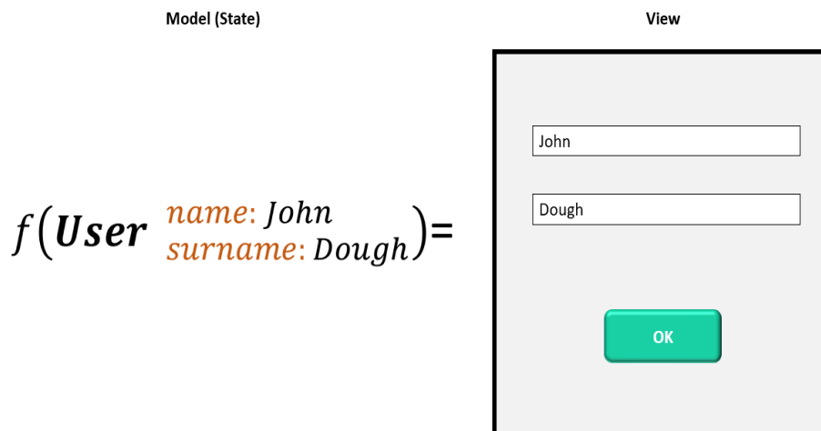
Figure 9. Declarative programming [Source: own]
