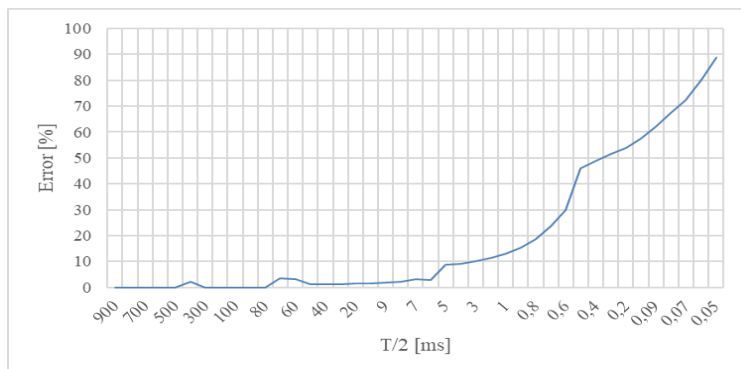
Figure 4. Frequency error values of microprocessor-generated signals
