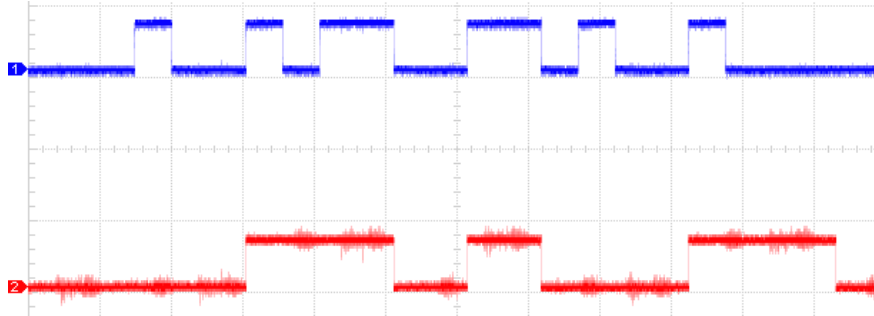
Figure 10. Encoded and decoded messages
