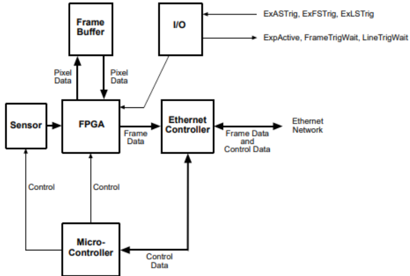
Figure 1. Block diagram of the camera [10]
