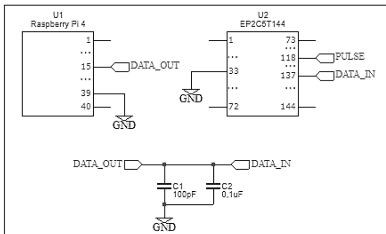
Figure 8. I/O points for LED control
