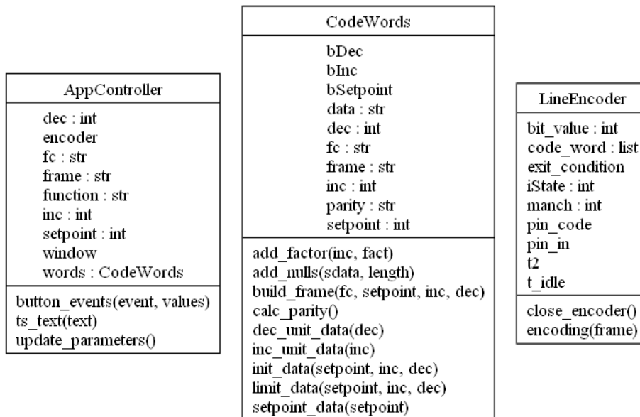
Figure 7. Class diagram of the application
