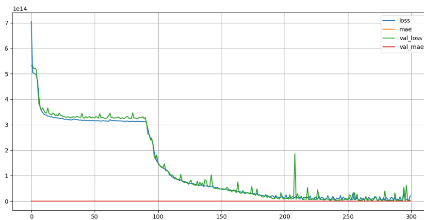
Figure 6. The training process of a 7-layer DNN
