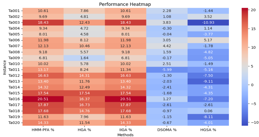
Figure 5. The average values of the test results of the Harmony Search algorithm
