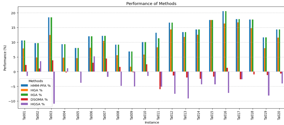
Figure 4. The average values of the test results of the Harmony Search algorithm. Figure 4 shows the average of Harmony Search test results, comparing them with the results published by the researchers in the form of a bar chart.
