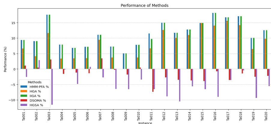
Figure 6. The average values of the test results of the Harmony Search algorithm
