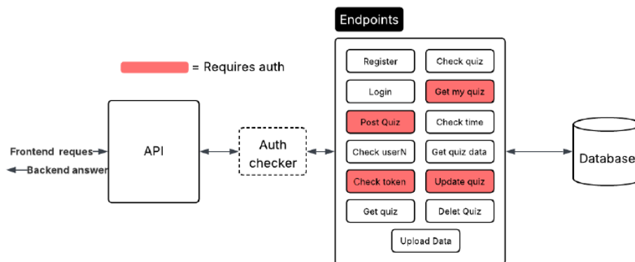
Figure 8. Backend structure
